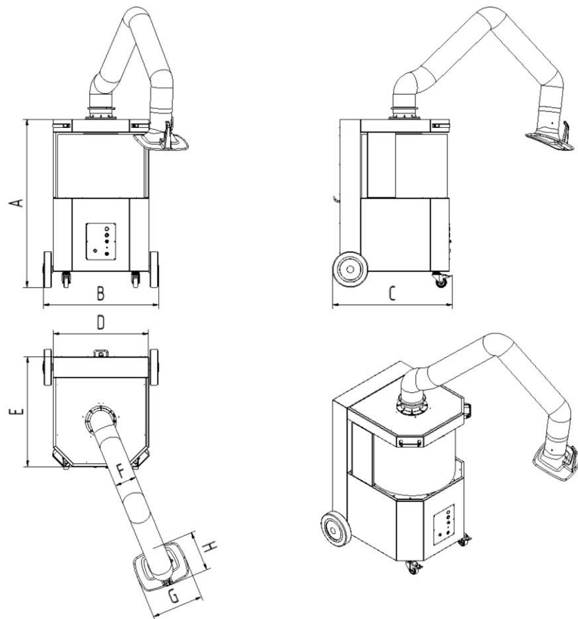
Fig. 7: Dimensions sheet
